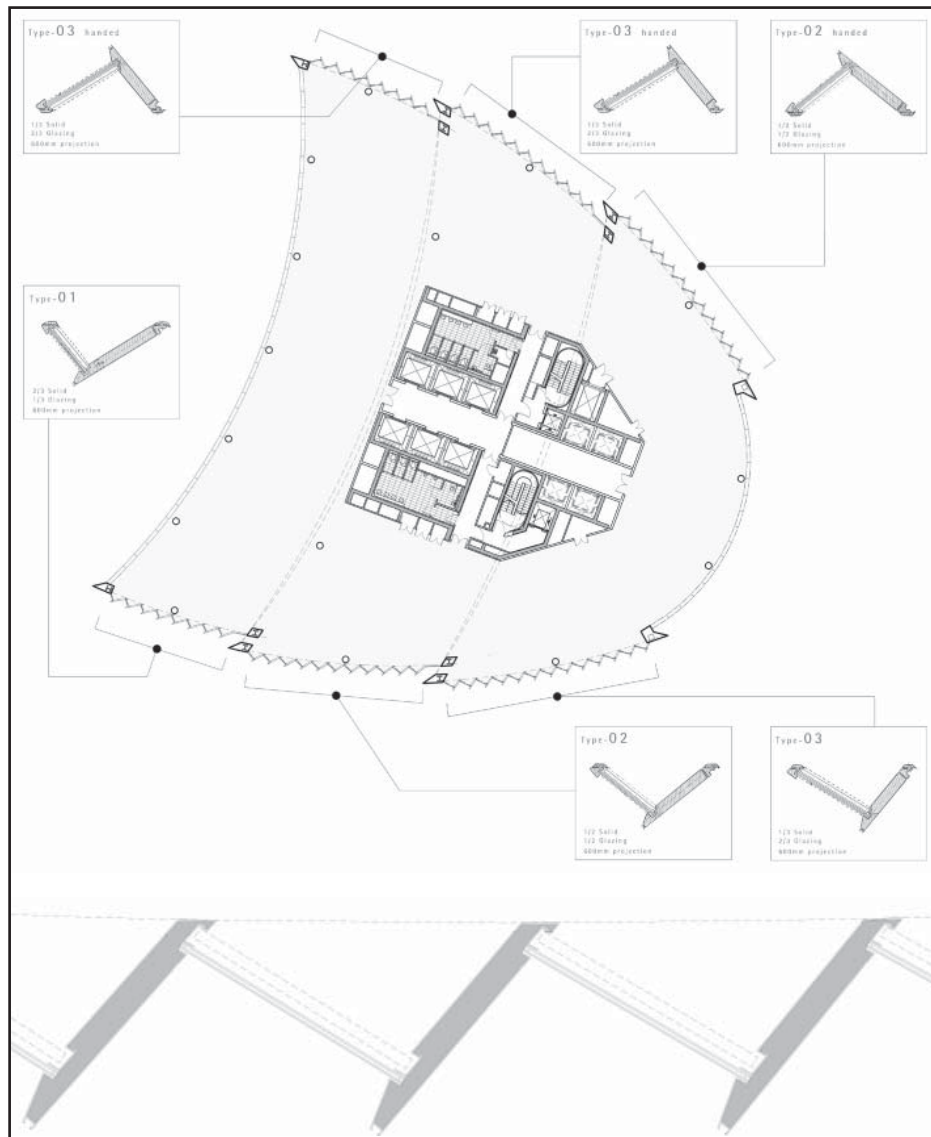
Cladding Typologies
